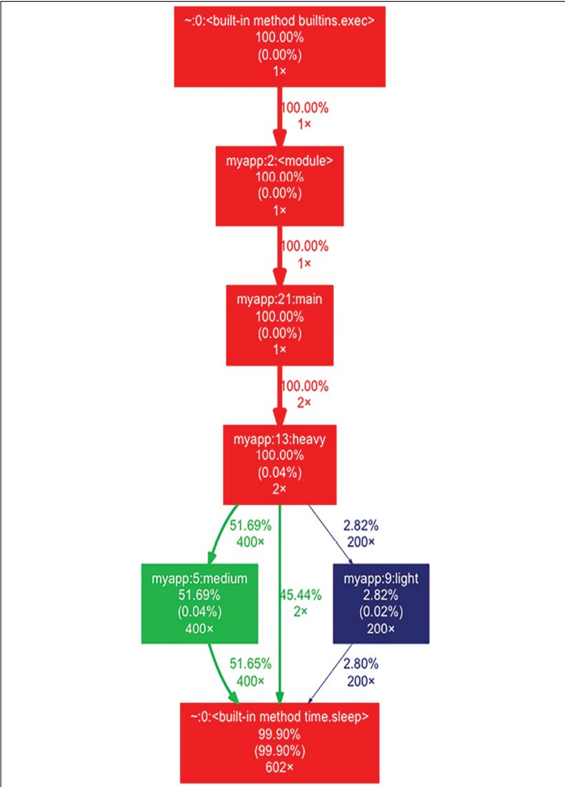
Figure 13.1: An example of a profiling overview diagram that was generated with gprof2dot
