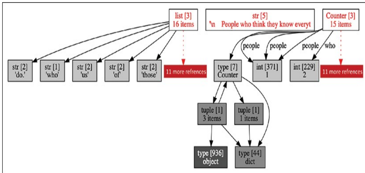
Figure 13.2: An example result of the show_refs() diagram from the graph_references() function
