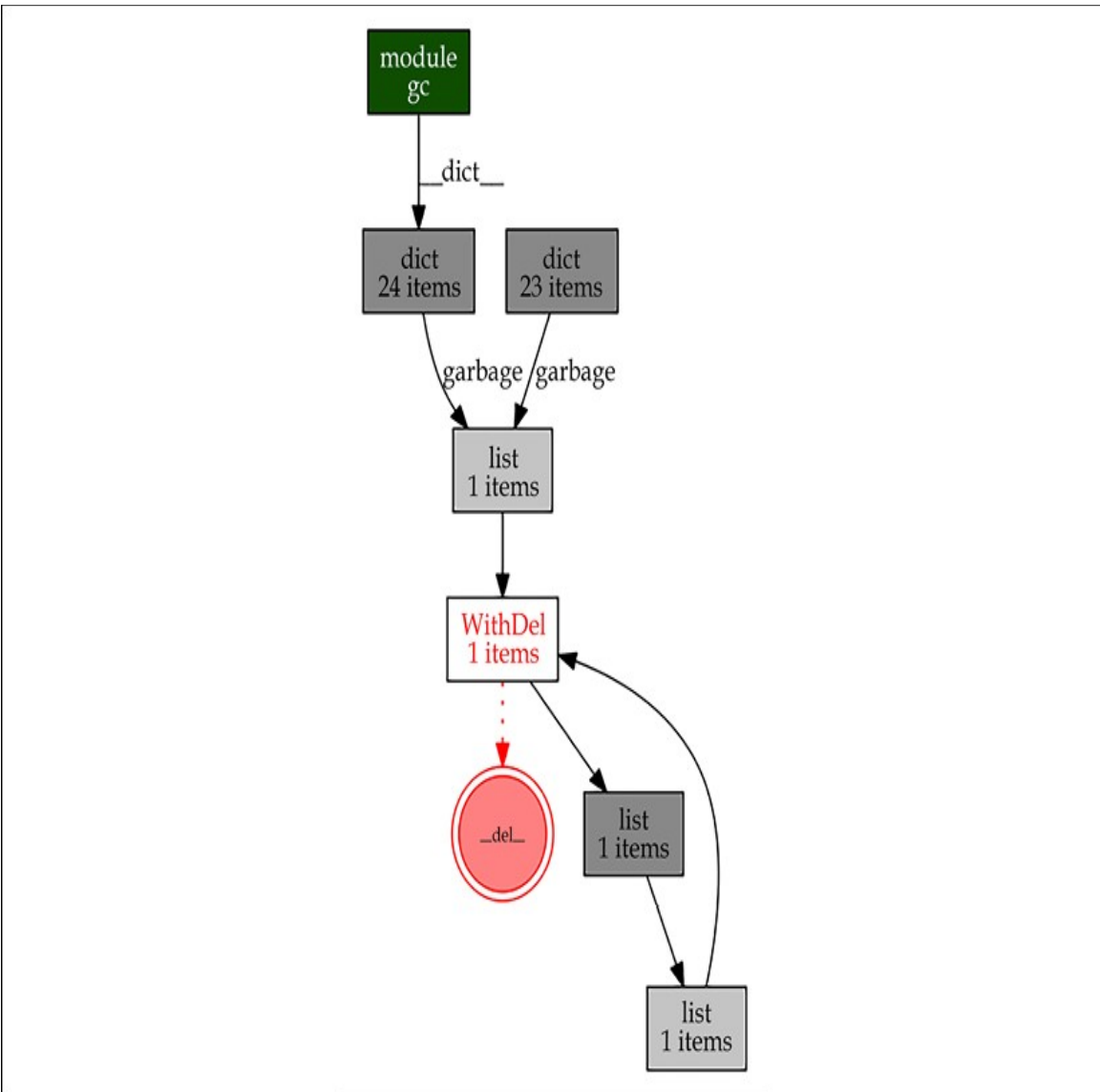
Figure 13.5: A diagram showing an example of cyclic references that can't be picked by the Python garbage collector prior to Python 3.4
