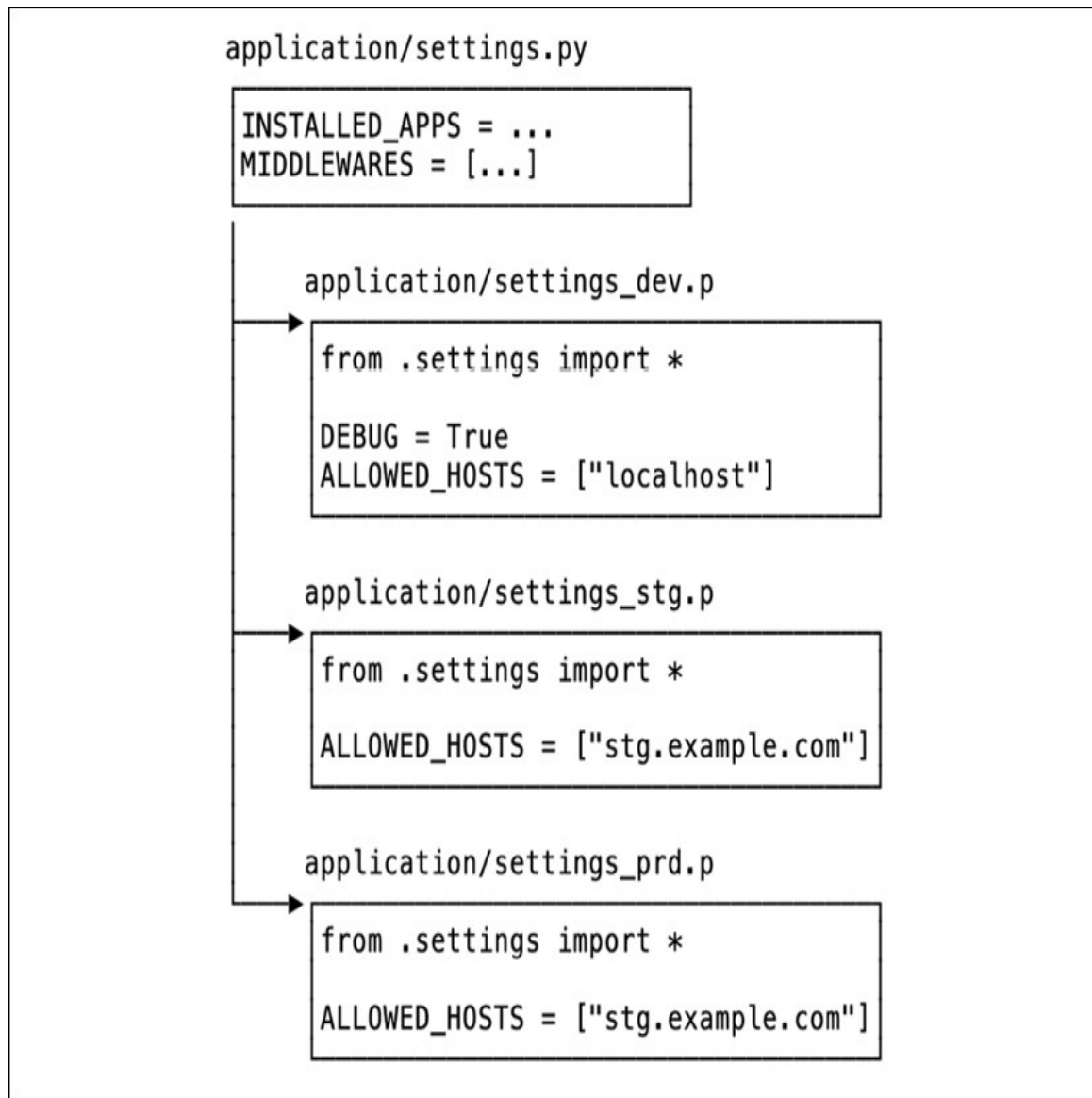
Figure 11.1: Typical layout of settings modules in many Django applications
