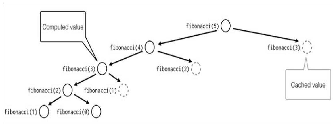
Figure 13.9: A call tree for the fibonacci(5) execution with memorization
