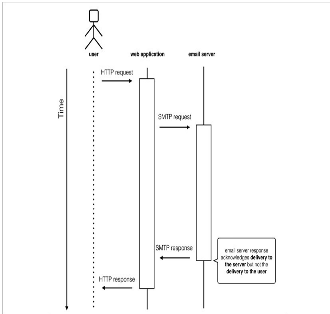
Figure 13.6: An example of synchronous email delivery in a web application
