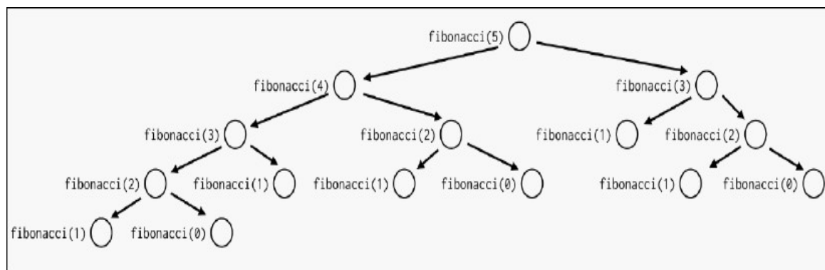
Figure 13.8: A call tree for the fibonacci(5) execution
