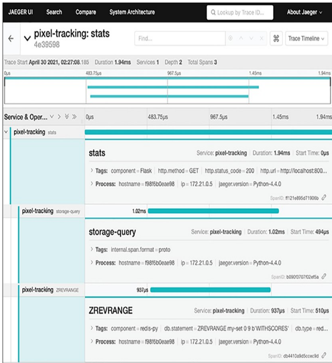
Figure 12.5: Example visualization of a distributed trace in the Jaeger web interface with multiple nested spans visible
