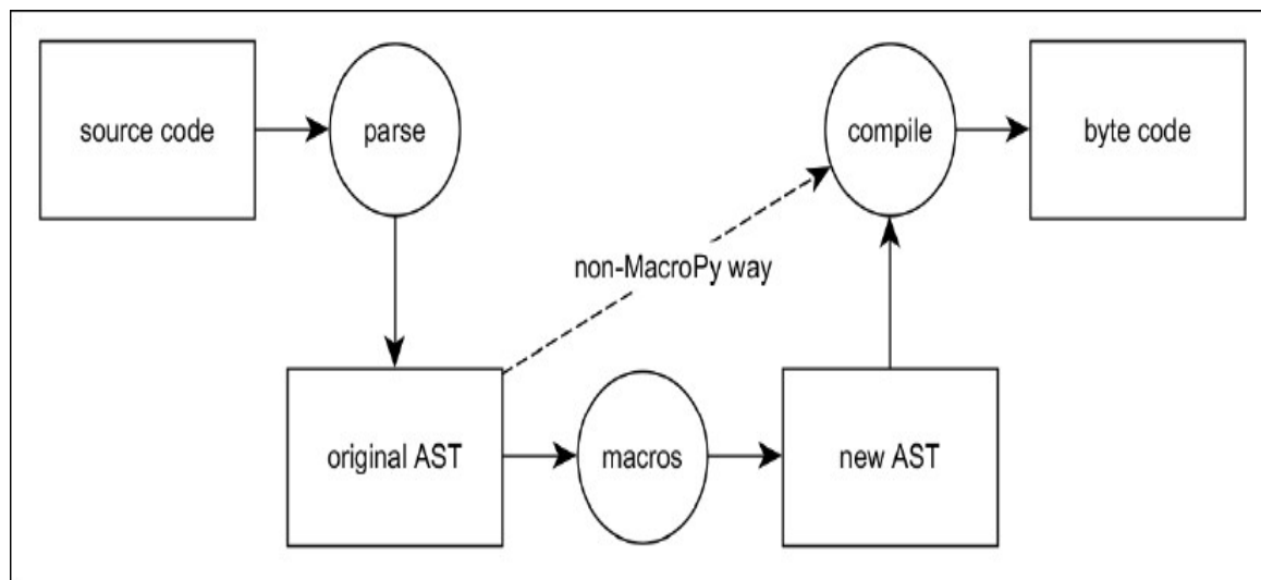
Figure 8.3: How MacroPy adds syntactic macros to Python modules on import
