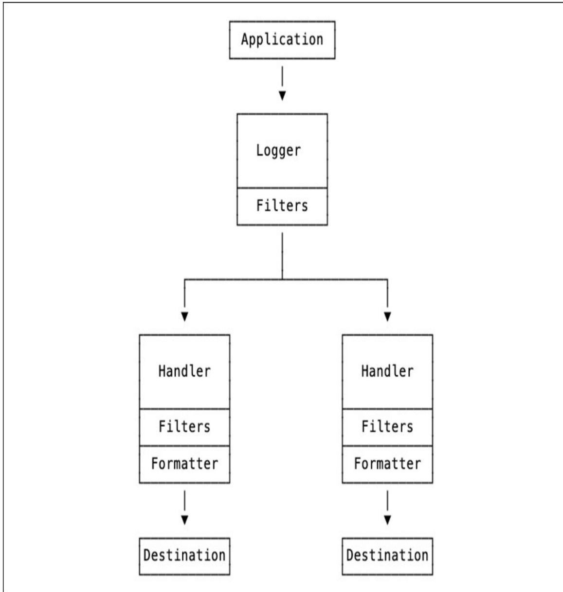
Figure 12.1: Topology of the Python logging system
