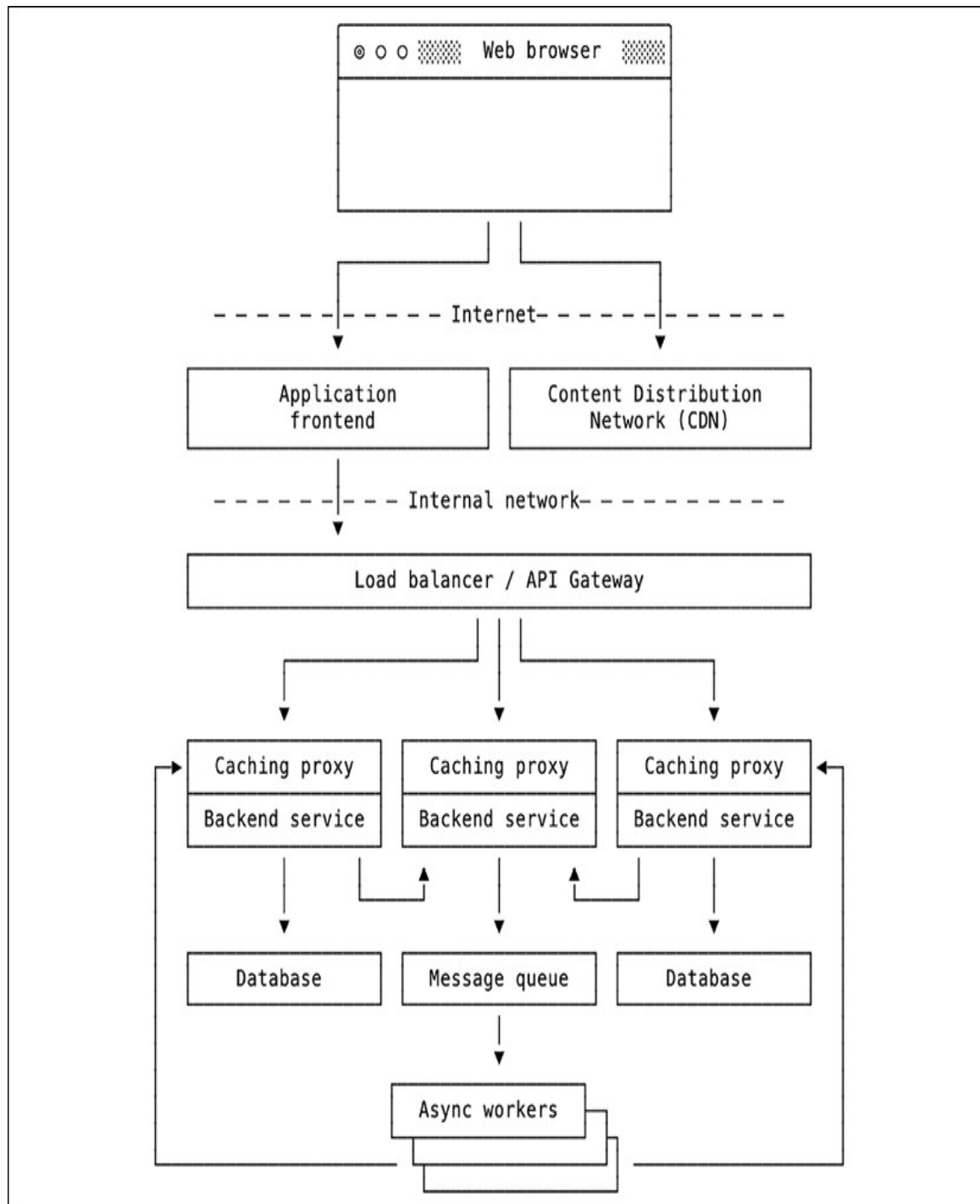
Figure 12.4: Example of an elaborate distributed application architecture with many inter-service connections
