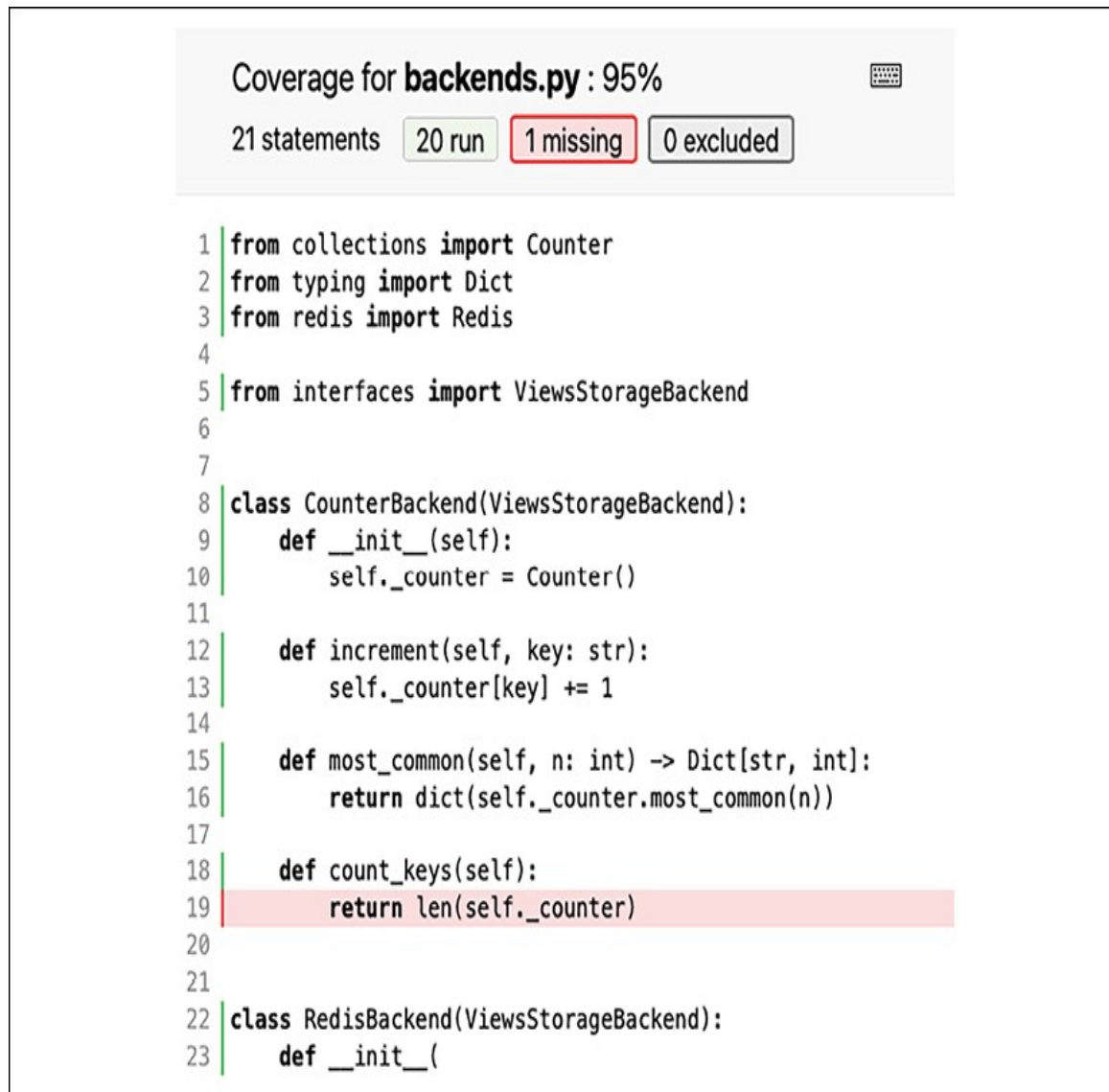
Figure 10.1: Example HTML coverage report highlighting coverage gaps
