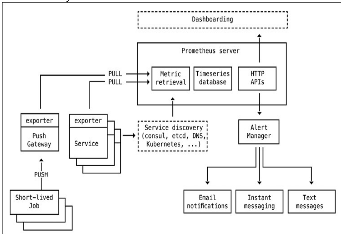
Figure 12.2: Architecture of a typical Prometheus deployment
