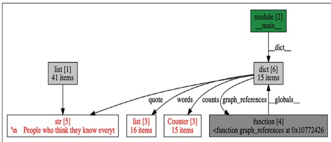
Figure 13.3: An example result of the show_backrefs() diagram from the graph_references() function
