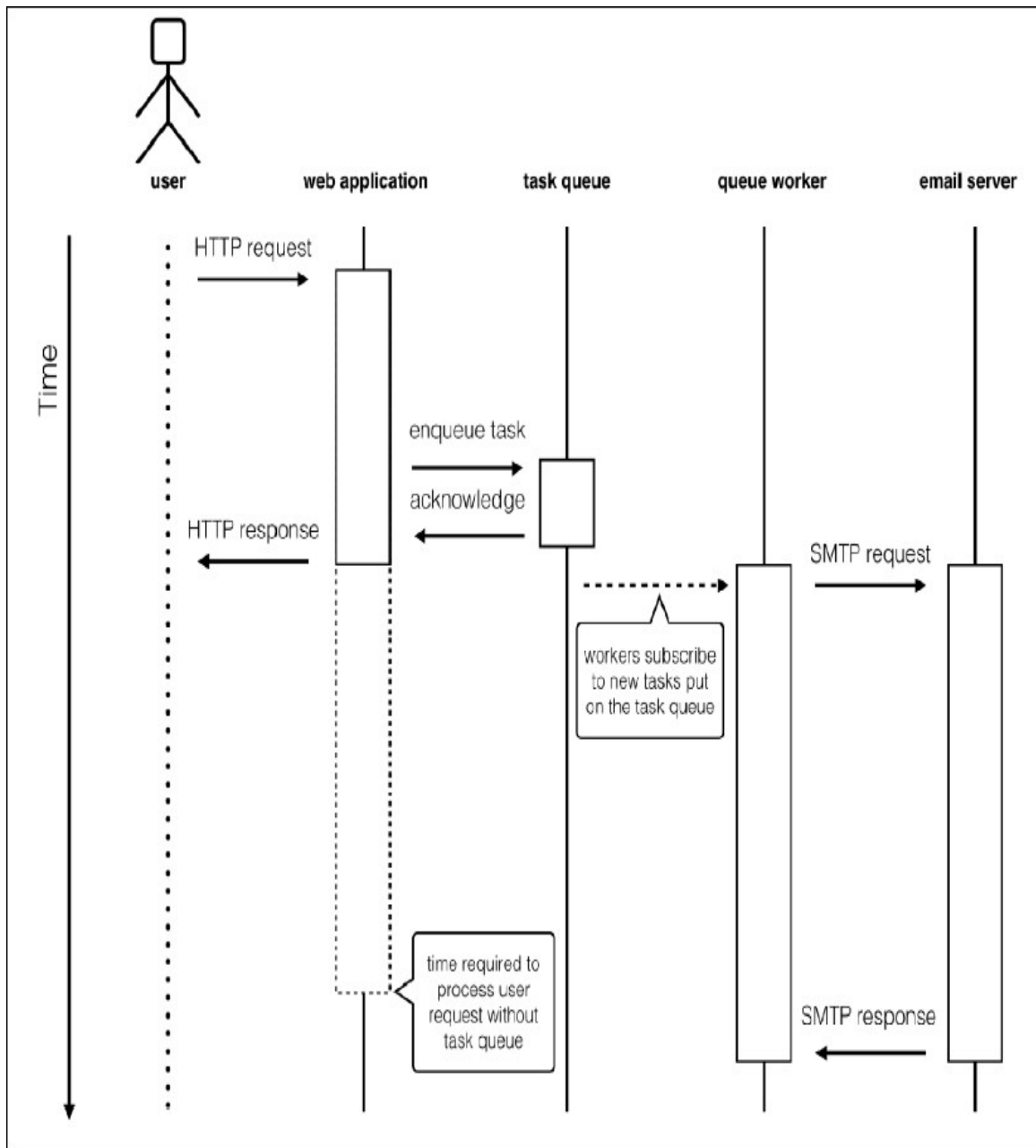
Figure 13.7: An example of asynchronous email delivery in a web application
