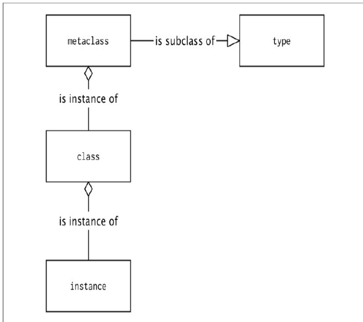
Figure 8.2: Usual implementation of custom metaclasses
