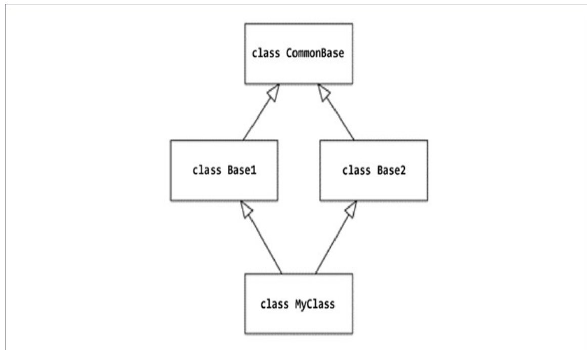
Figure 4.2: The diamond class hierarchy
