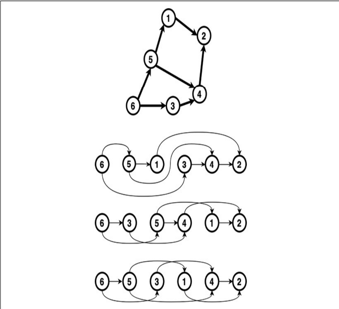
Figure 3.2: Various ways to sort the same graph topologically
