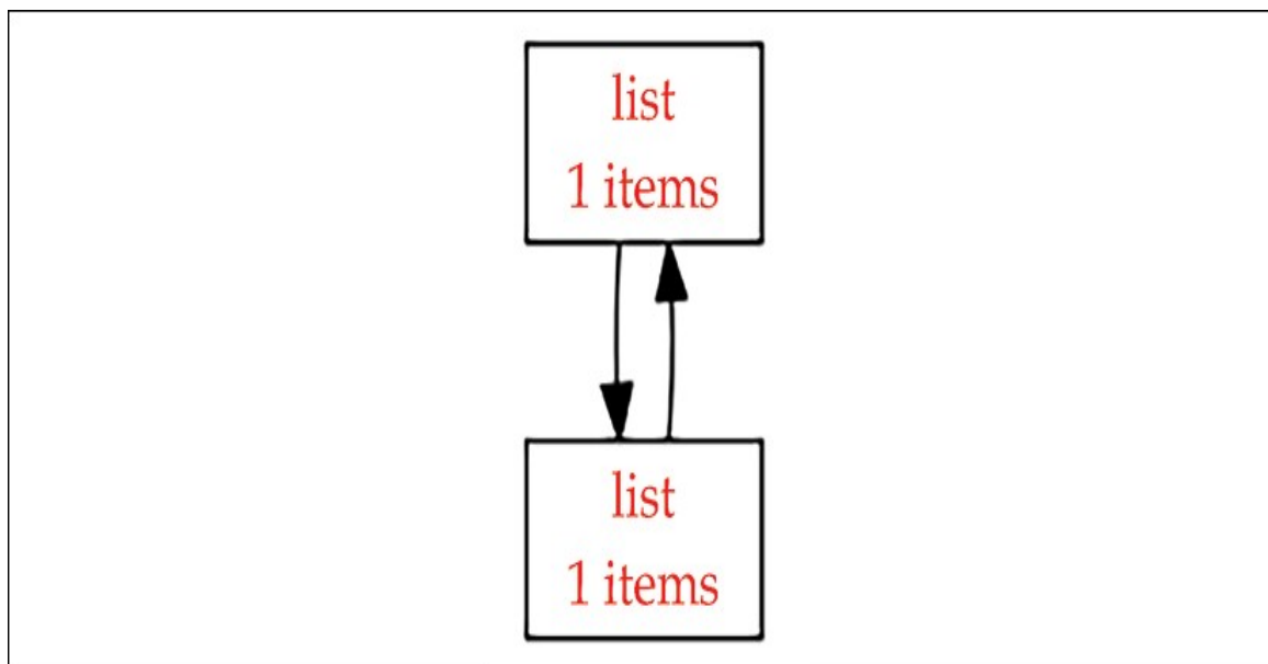
Figure 13.4: An example diagram generated by objgraph of cyclic references between two objects
